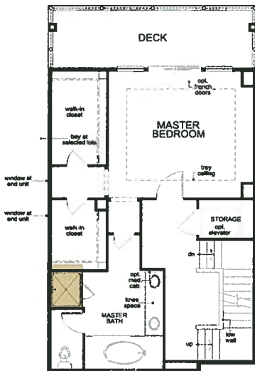
alternate third floor plan
